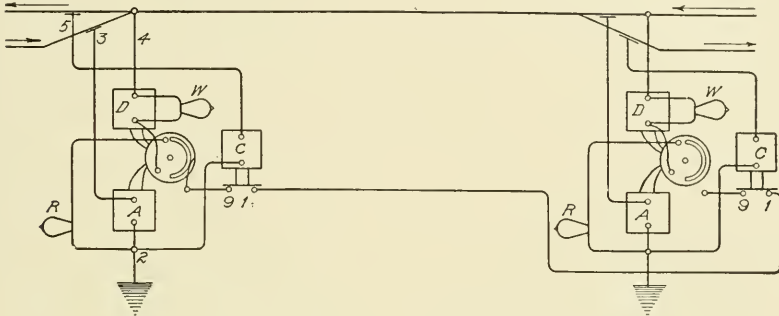
Fig. 213. Diagram of Automatic Block Signal System
